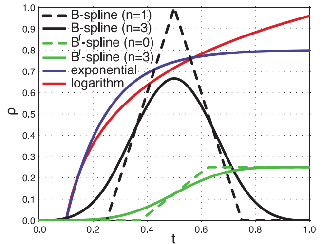
Figure 2. Basis functions used in the time-dependent parametrization of ground deformation. B-splines and B ∫ -splines have uniform knot spacing of 0.25, and only the basis centered at 0.5 is shown.
