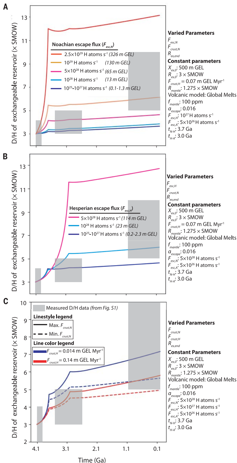
Fig. 2. Simulated D/H evolution for different assumptions of crustal hydration and atmospheric escape rates. (A to C) The evolution of the D/H of the exchangeable reservoir in our simulation.
