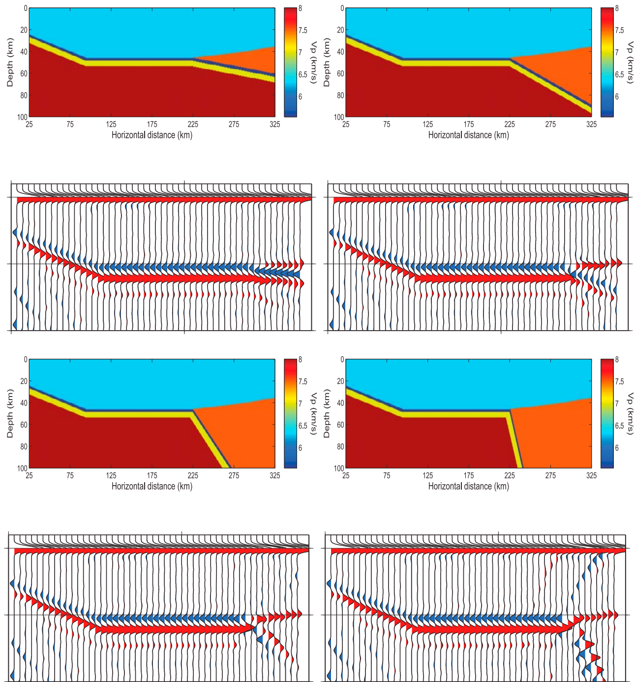
Figure 12. Dip sensitivity test results using 2-D finite difference modeling to demonstrate that RFs at steeper angles do not work. The dip angles vary from 10^\circ , 25^\circ , 50^\circ , to 75^\circ . Note that the polarity of the synthetic RFs changes the sign when the dip angle exceeds 50^\circ . Also, the diffraction artifact from a sharp corner appears to be strong in the overlying crust.
