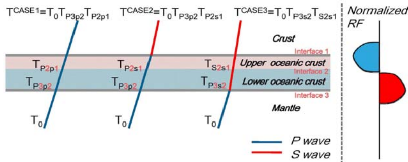
Figure 13. Schematic showing transmitted responses at top and bottom interfaces of the oceanic crust. The RF responses responses are normalized by the P arrival. The peak of the negative RF pulse is obtained at the interface 1 between the crust and the upper oceanic crust; the peak of the positive RF pulse at the interface 3 between the lower oceanic crust and the mantle.
