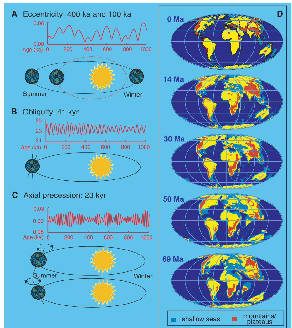
Fig. 1. Primary orbital components are displayed on the left, and Cenozoic paleogeography on the right. The gravitational forces exerted by other celestial bodies affect Earth’s orbit. As a result, the amount and, more importantly, the distribution of incoming solar radiation oscillate with time (123). There are three orbital perturbations with five periods: eccentricity (at 400 and 100 ky), obliquity (41 ky), and precession (23 and 19 ky). (A) Eccentricity refers to the shape of Earth’s orbit around the sun, varying from near circular to elliptical. This effect on insolation is very small, however, and by itself should not account for changes in Earth’s climate during the past. (B) Obliquity refers to the tilt of Earth’s axis relative to the plane of the ecliptic varying between 22.1^\circ and 24.5^\circ . A high angle of tilt increases the seasonal contrast, most effectively at high latitudes (e.g., winters in both hemispheres will be colder and summers hotter as obliquity increases). (C) Precession refers to the wobble of the axis of rotation describing a circle in space with a period of 26 ky. Modulated by orbital eccentricity, precession determines where on the orbit around the sun (e.g., with relation to aphelion or perihelion) seasons occur, thereby increasing the seasonal contrast in one hemisphere and decreasing it in the other. The effect is largest at the equator and decreases with increasing latitude. The periods of the precessional signal modulated by eccentricity are 23 and 19 ky, the periods observed in geological records. (D) Continental geography reconstructed for five intervals of the last 70 My (designed using the commercial Paleogeographic Information System).
