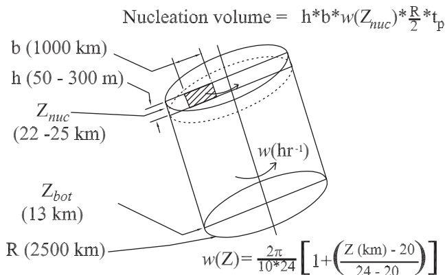
Figure 1. Schematic diagram of the domain used to simulate the polar vortex region (expressions for angular velocity and nucleation volume are also listed). Particles are seeded in a nucleation layer at Z_{nuc} and tracked as they sediment to Z_{bot} . Angular velocity is chosen such that a 2\pi revolution takes 5 days at 24 km altitude and 10 days at 20 km altitude.
