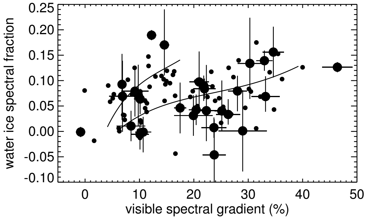
Fig. 3.— Water ice absorption fraction as a function of spectral color gradient. Black points with error bars show the spectra data and colors derived from visible photometry. The red points without error bars (typical uncertainties are smaller than those of the spectral data) are from the H/WTSOSS photometric survey of Fraser & Brown (2011) and have been transformed to these variables. The two lines show the mixing models which best fit the three-color H/WTSOSS data. The blue and red shading show the neutral and the red families of objects.
