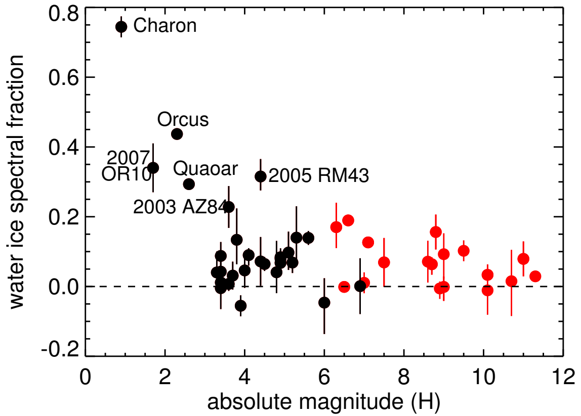
Fig. 2.— Water ice absorption as a function of absolute magnitude. Objects with semimajor axis outside of 30 AU are shown in black, while those inside of 30 AU are shown in red.
