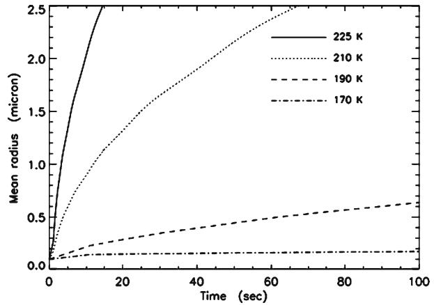
Fig. 1 The growth of water ice corresponding to conditions on Enceladus for a variety of cases are shown. We see that particles can grow much more quickly with increasing water vapor abundance. To grow \sim 1 \mu\text{m} plume particles in the time frame of tens of seconds, we need a minimal water vapor abundance of \sim 10^{13} \text{ molecules cm}^{-3} corresponding to a minimal saturation density at \sim 190 \text{ K}
