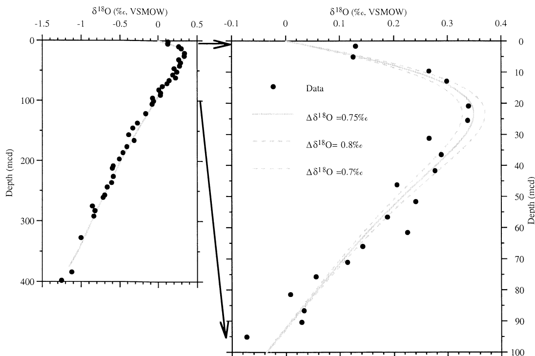
Figure 2. Plot of \delta^{18}\text{O} vs. meters composite depth in ODP core 1063A. Error bars ( 1\sigma ) are from replicate analyses of the same sample. The gray line is the best-fit model run using a glacial/interglacial change of 0.75\text{‰} . Dashed gray lines are the results of changing the 0.75\text{‰} fit by \pm 0.05\text{‰} .
