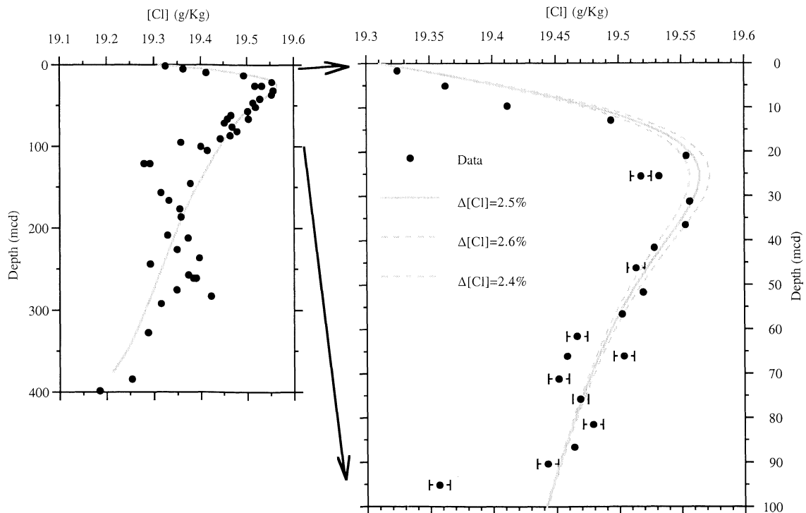
Figure 1. Plot of [Cl] vs. meters composite depth in ODP core 1063A. Error bars ( 2\sigma ) are the propagated uncertainties from weighing, titration volume, and standard calibration. Replicate analyses generally agree within errors. The gray line is the best-fit result from a 1-D diffusion model that includes compaction advection and has a glacial to interglacial change of 2.5%. Dashed gray lines are two other fits that bracket the ideal result by 0.1%.
