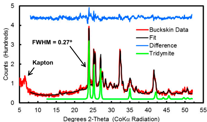
Fig. 2. Buckskin diffraction pattern (red) from sum of first four diffraction images, calculated pattern from Rietveld analysis (black), difference pattern (blue), and refined tridymite pattern (offset green); see SI Appendix, Fig. S4 for refined patterns of all minerals. Full width at half maximum intensity (FWHM) of the tridymite peak at 23.9^\circ 2\theta is 0.27^\circ 2\theta , which corresponds to CheMin 2\theta resolution measured on Earth before launch (ref. 4, figure 18). Peak at \sim 6.5^\circ 2\theta is from the Kapton cell window.
