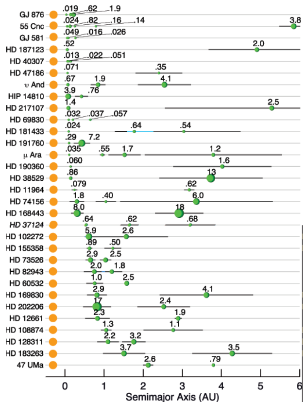
FIG. 4.— Chart showing the semimajor axes and minimum masses for the 31 known planetary systems containing more than 1 planet (data from Wright et al. [2009], as updated by Correia et al. [2009], Mayor et al. [2009] and Niedzielski et al. (2009)). The horizontal lines under each planet indicate the distance between periape and apoapse for eccentric orbits. The sizes of the planet symbols scale as (M_P \sin i)^{1/3} , and the labels denote the planet mass in units of M_{Jup} .
