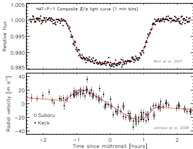
FIG. 3.— Transit observations of the exoplanet HAT-P-1b, which was discovered by the HAT-Net wide-field transit survey (Bakos et al. 2007). The planet has a mass M_P = 0.53 M_{\text{Jup}} , and an orbital period P = 4.465 days. Upper : A composite transit light curve constructed from 7 individual photometric data sets (Winn et al. 2007). The photometry was phased by subtracting the mid-transit time from each light curve. The best-fitting model gives a planet radius R_P = 1.225 \pm 0.056 R_{\text{Jup}} . Lower : Phased radial velocity measurements made during three transits, illustrating the Rossiter-McLaughlin (RM) effect. The shape of the RM waveform yields the projected spin-obit angle. The HAT-P-1 planetary system is well aligned with a spin-obit angle of 3.7 \pm 2.1 degrees (Johnson et al. 2008).
