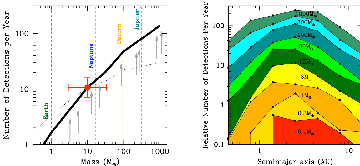
Fig. 2.— Expectations from the next generation microlensing survey, including MOA-II, OGLE-IV, and a Korean telescope in South Africa. (Left) Number of planets detected per year, normalized to number of \sim 10M_{\oplus} found to date by microlensing (indicated by the red dot). The solid line is the prediction assuming an equal number of planets per logarithmic mass interval, and the dotted grey curve assumes that the number of planets per log mass scales as m^{-1/3} . Planets are assumed to be distributed uniformly in \log(a) between 0.4–20 AU. Arrows indicate the locations of 8 published exoplanets plus one unpublished planet (Sumi et al. 2009). (Right) The semi-major axis distribution of the detected planets.
